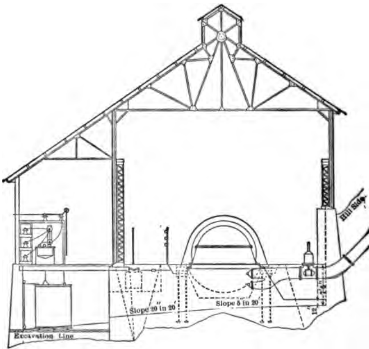
FIG. 16.— SHOWING GENERAL ARRANGEMENT OF POWER-HOUSE.
